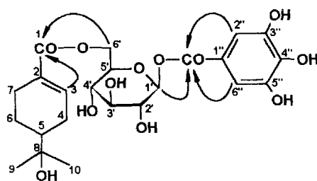
FIGURE 1 The key correlations of 1 in HMBC spectrum.
